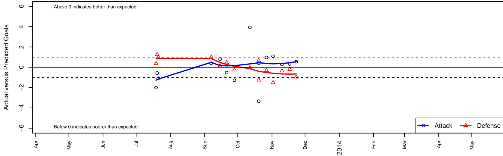
Strikers FC Whittier B97 Dots are actual minus expected GF (blue circles) and GA (red triangles). Blue line is smoothed change in attack strength. Red is smoothed change in defense strength.
